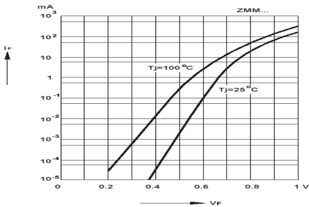
Forward characteristics
