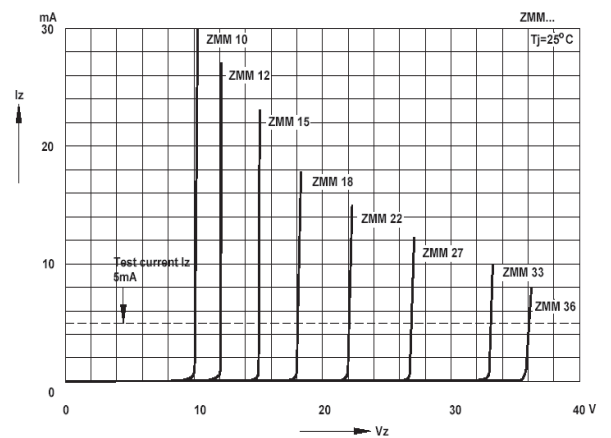
Breakdown characteristics at T_J = \text{constant} (pulsed)
