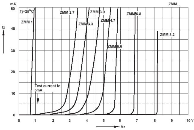
Breakdown characteristics at T_J = \text{constant} (pulsed)
