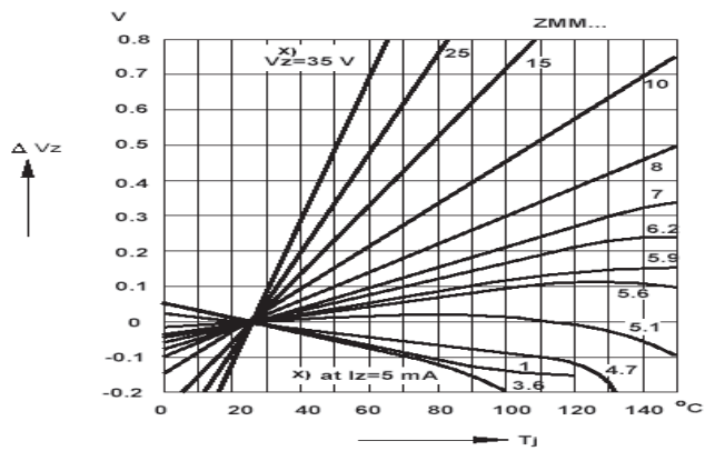
Change of Zener voltage versus junction temperature
